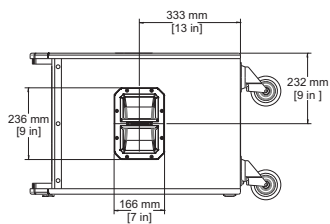
Right View
